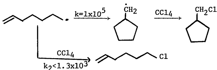
Scheme XII
