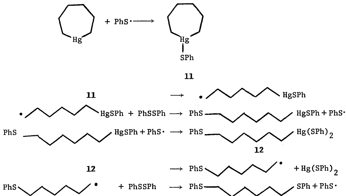
Scheme XIX
